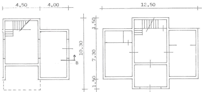
'A PIANO SEMINTERRATO
